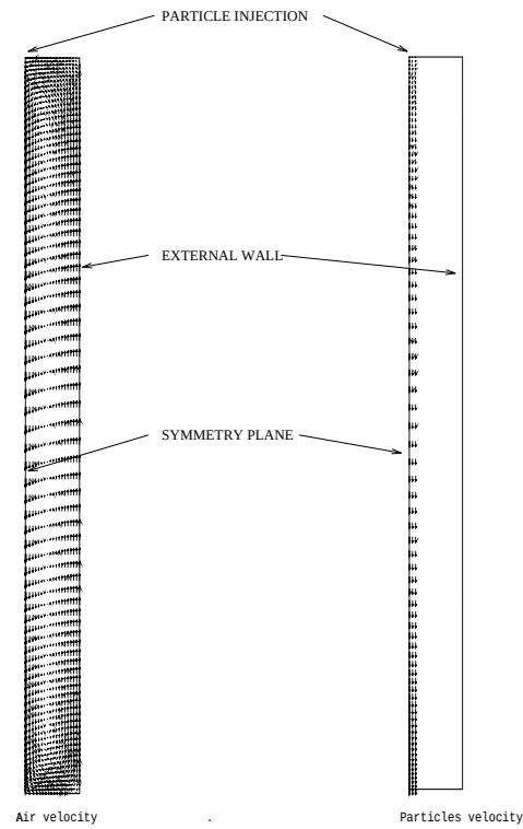
FIG. 4.2.2 – Test case 35/500. Computed air and particles velocity
