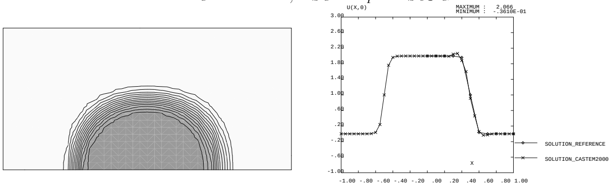
FIG. 1.1.4 – Cas \nu = 10^{-6} , TSCAL option SUPG
