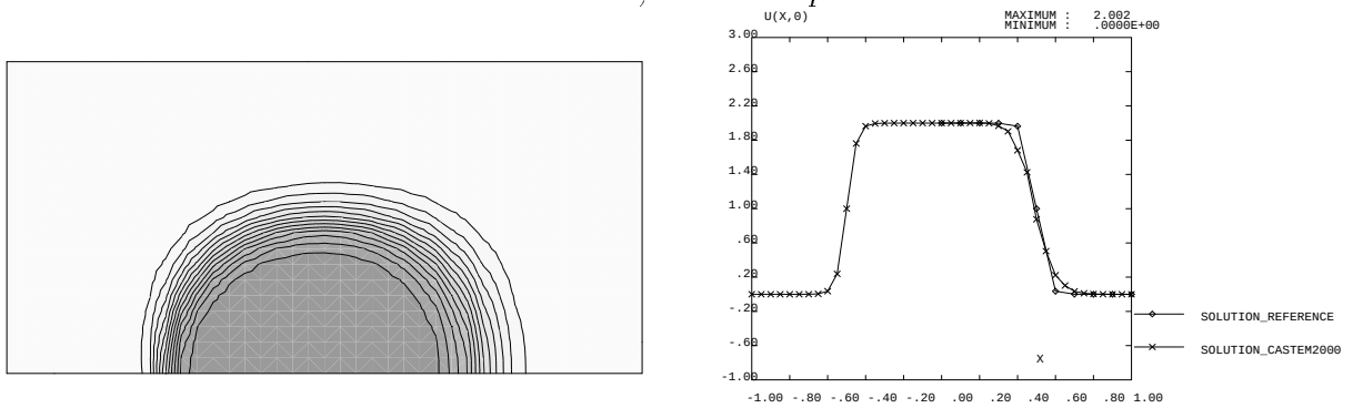
FIG. 1.1.5 – Cas \nu = 10^{-6} , TSCAL option SUPG-CC
