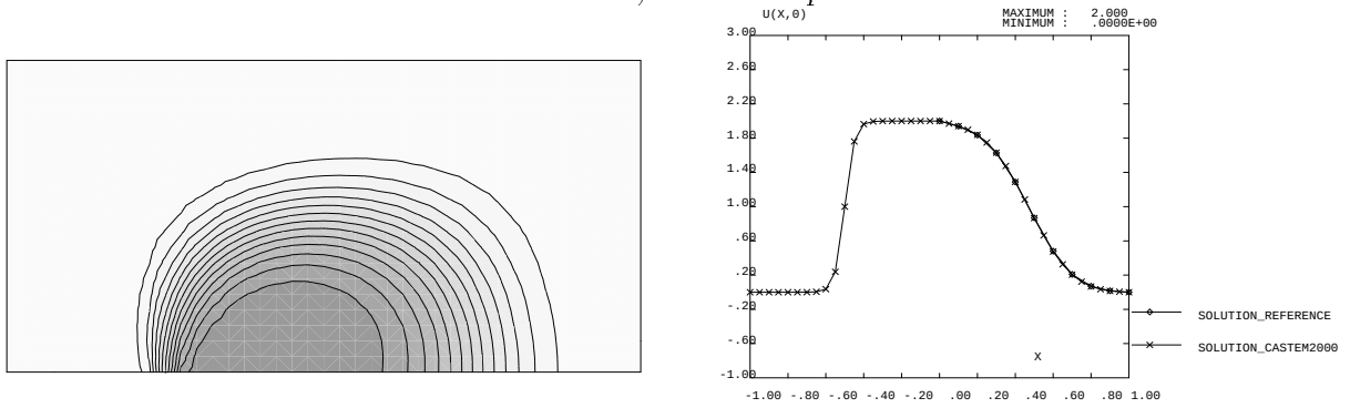
FIG. 1.1.3 – Cas \nu = 10^{-2} , TSCAL option SUPG
