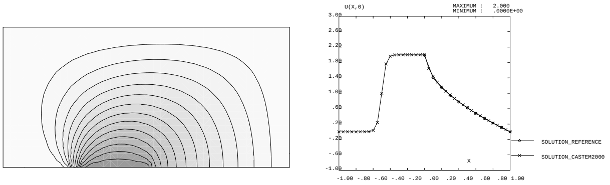
FIG. 1.1.2 – Cas \nu = 10^{-1} , TSCAL option SUPG
