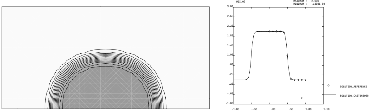
FIG. 1.1.8 – Cas \nu = 10^{-6} , EFMH implicite , maillage \square
