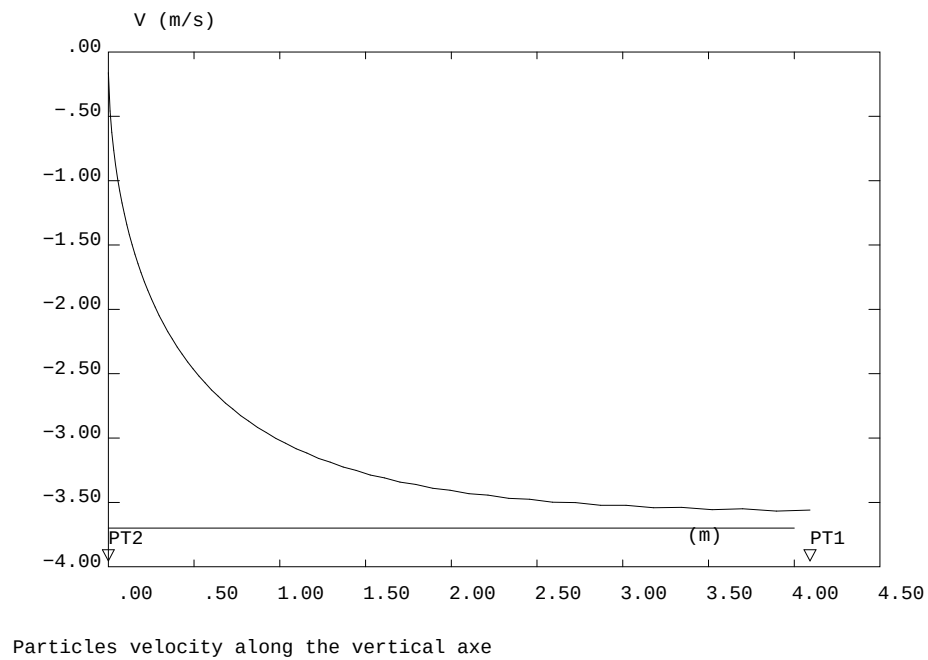
FIG. 4.1.1 – Particle velocity along the vertical axis compared with the limit velocity.
