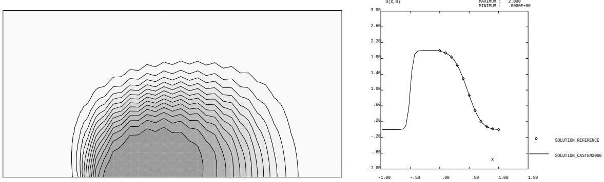
FIG. 1.1.10 – Cas \nu = 10^{-2} , EFMH implicite, maillage \Delta
