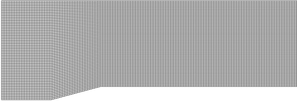
MAILLAGE 180x60
