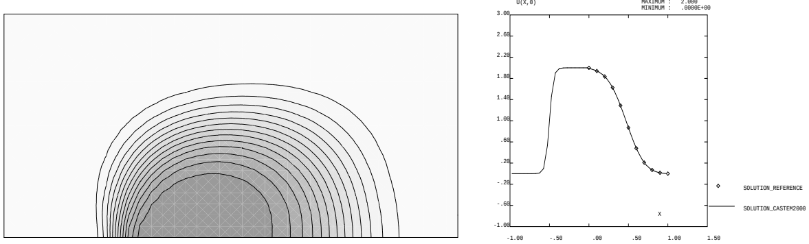
FIG. 1.1.7 – Cas \nu = 10^{-2} , EFMH implicite , maillage \square
